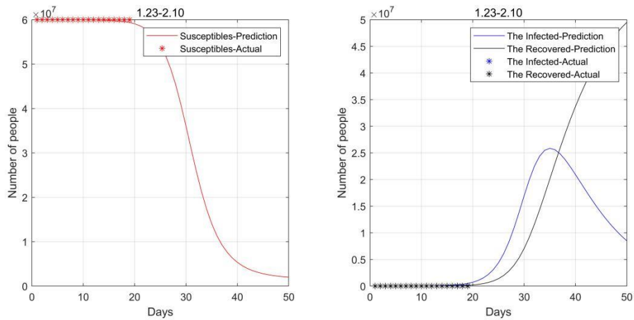
Fig. 3. 2020.1.23-2020.2.10 Data fitting result (consider birth rate and natural mortality).
