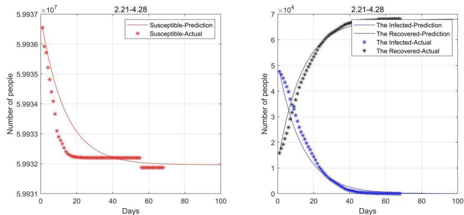
Fig. 6. 2020.2.21-2020.4.28 Data fitting result (not consider birth rate and natural mortality).
