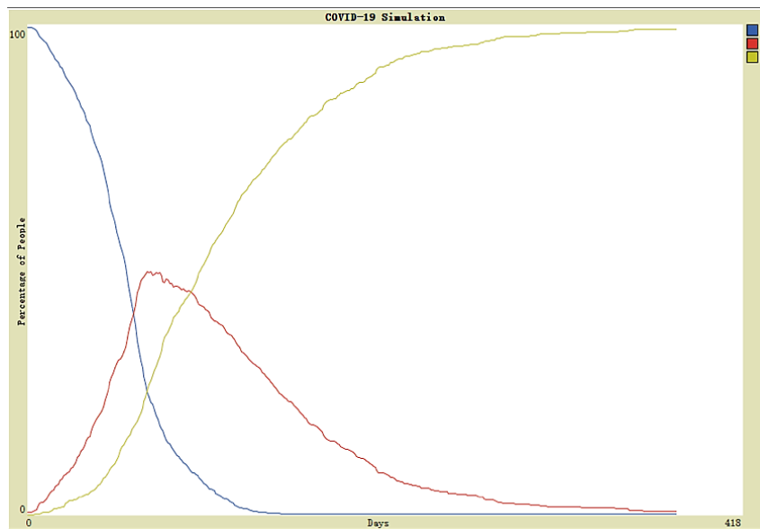
Fig. 8. Simulation fitting result from Netlogo.
