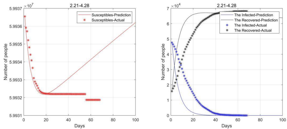
Fig. 4. 2020.2.21-2020.4.28 Data fitting result (consider birth rate and natural mortality).
