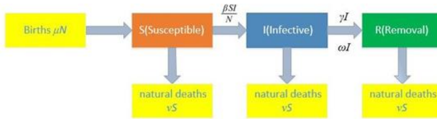
Fig. 1: SIR model diagram in Hubei Province (consider births and natural deaths).
