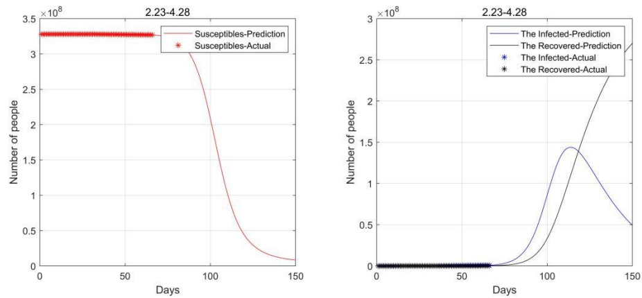
Fig. 7. 2020.2.23-2020.4.28 Data fitting result (not consider birth rate and natural mortality).
